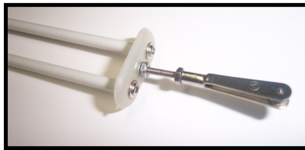
Diagram 3 - Elevator pushrod joiner
